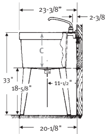
Floor Model 23-3/8" D x 21-5/8" W (594 mm x 549 mm) A 20-3/4", B 19-1/4", C 13-1/4"
